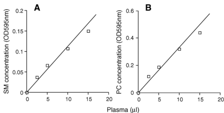
Fig. 3. Linear ranges of plasma SM and PC measurements. Pooled human plasma was used. Different amounts of the plasma supplemented with saline to 20 \mu l were incubated with a 100 \mu l reaction buffer at 37°C for 45 min, and absorption was measured at 595 nm. A: Plasma linear range for SM measurement. B: Plasma linear range for PC measurement. OD, optical density.
